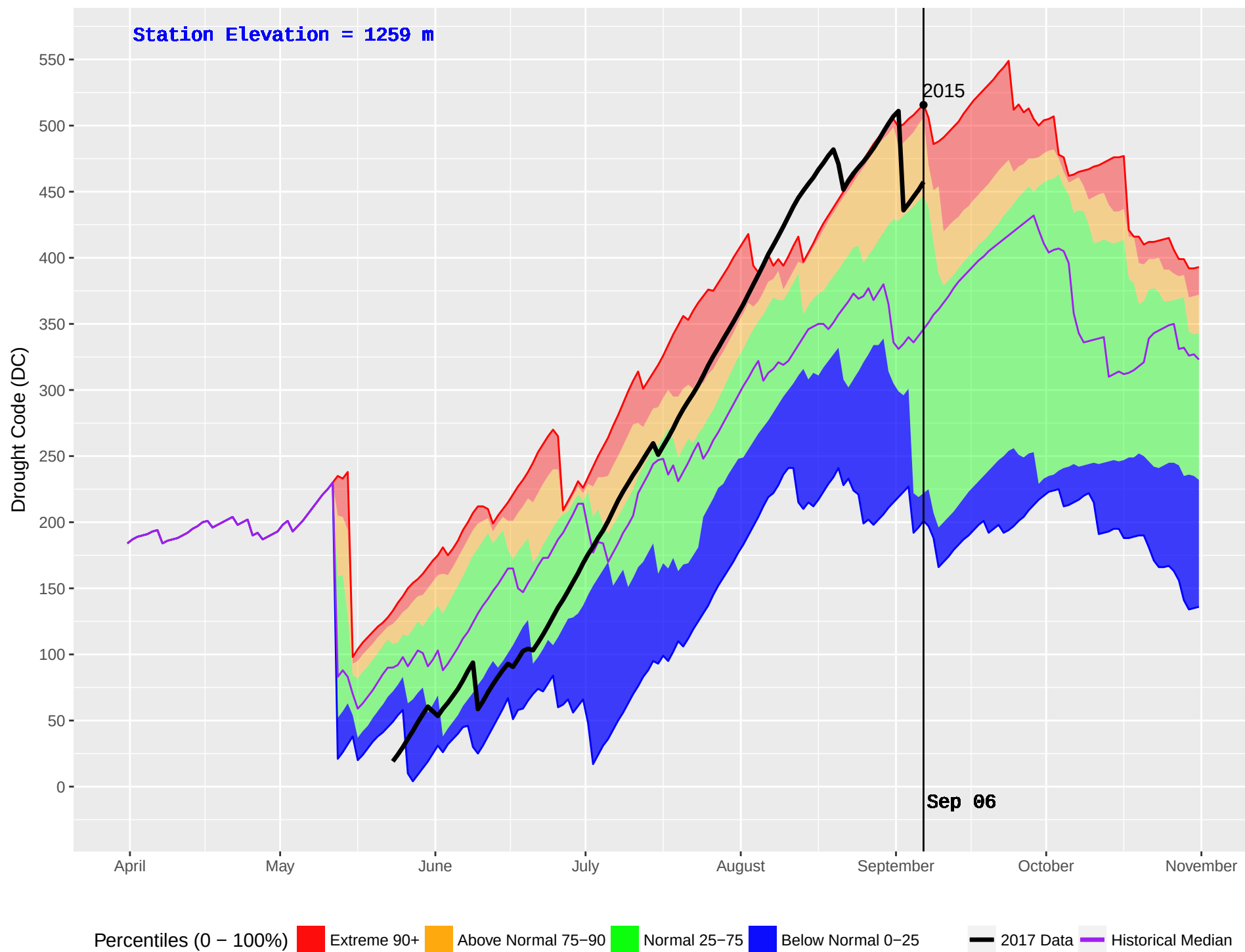
PARROTT (183) : Historical (1995–2016) and Current (2017) Noon Drought Code (DC)
