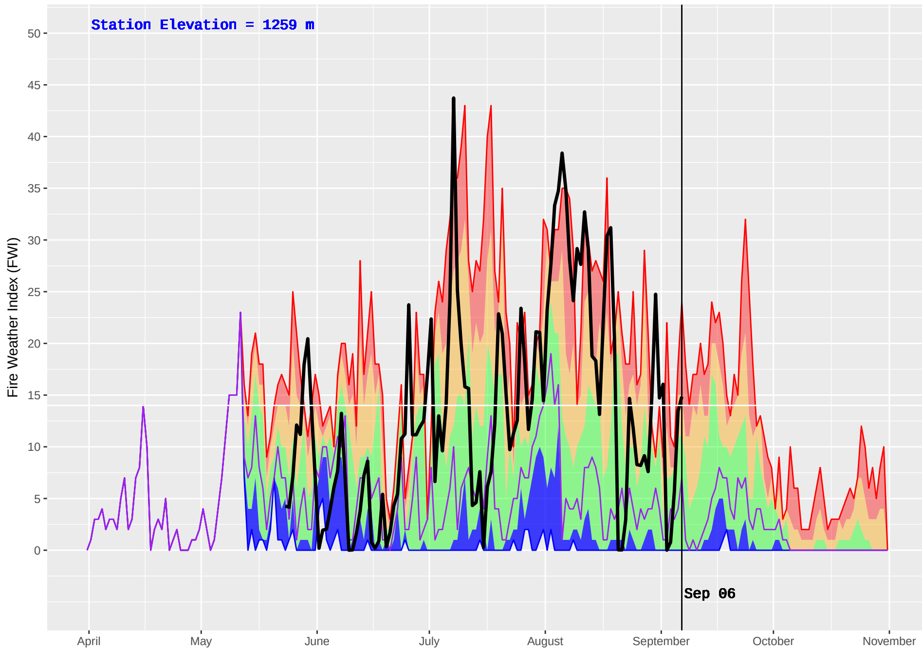
PARROTT (183) : Historical (1995–2016) and Current (2017) Noon Fire Weather Index (FWI)
