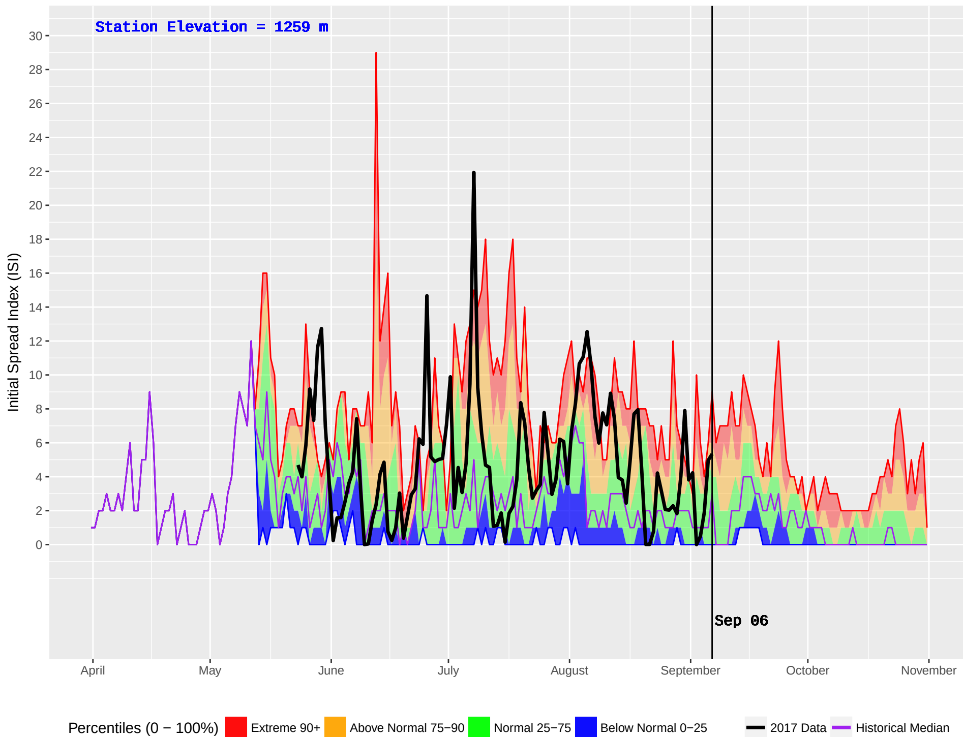
PARROTT (183) : Historical (1995–2016) and Current (2017) Noon Initial Spread Index (ISI)
